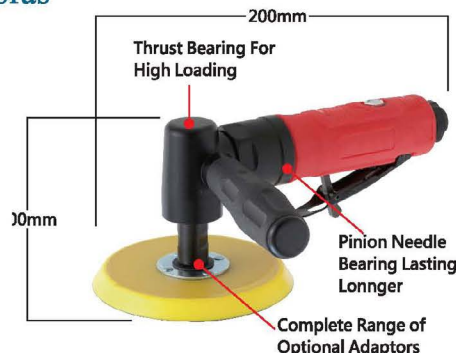
Multi-Function Angle Sander/Polisher
